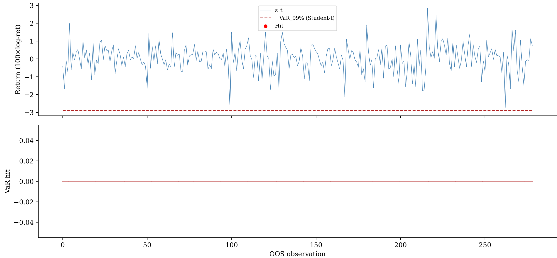
LSTM-SSE-t-Student — SP500 VaR 99% Hit Sequence
